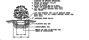
3 SHRUB PLANTING DETAIL SCALE: NOT TO SCALE
