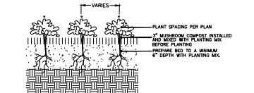
2 ANNUAL, PERENNIAL & GROUND COVER DETAIL SCALE: NOT TO SCALE
