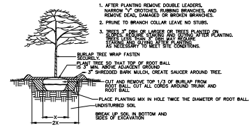
4 TREE PLANTING DETAIL SCALE: NOT TO SCALE
