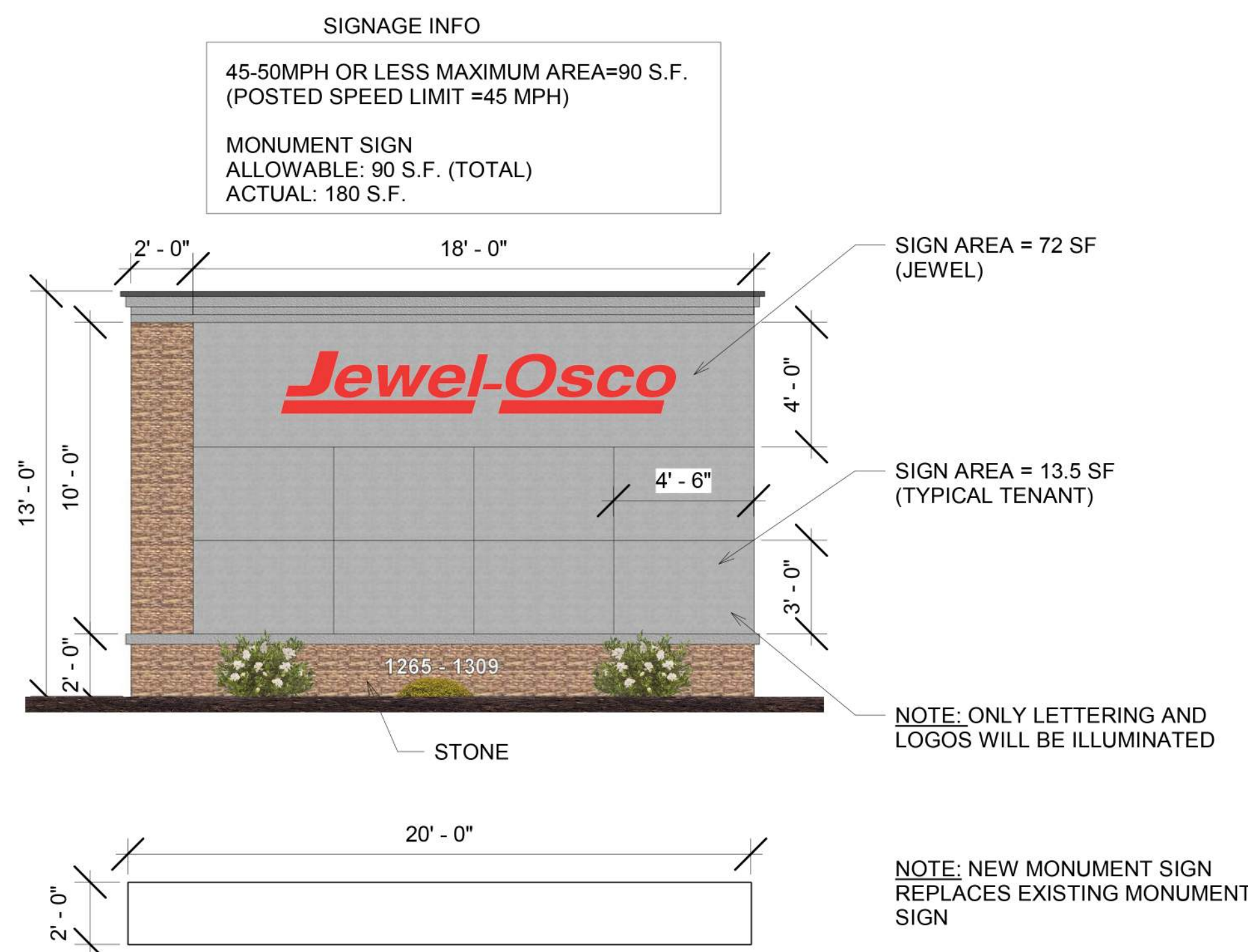
4 PROPOSED MONUMENT SIGN 2 1/4" = 1'-0"
