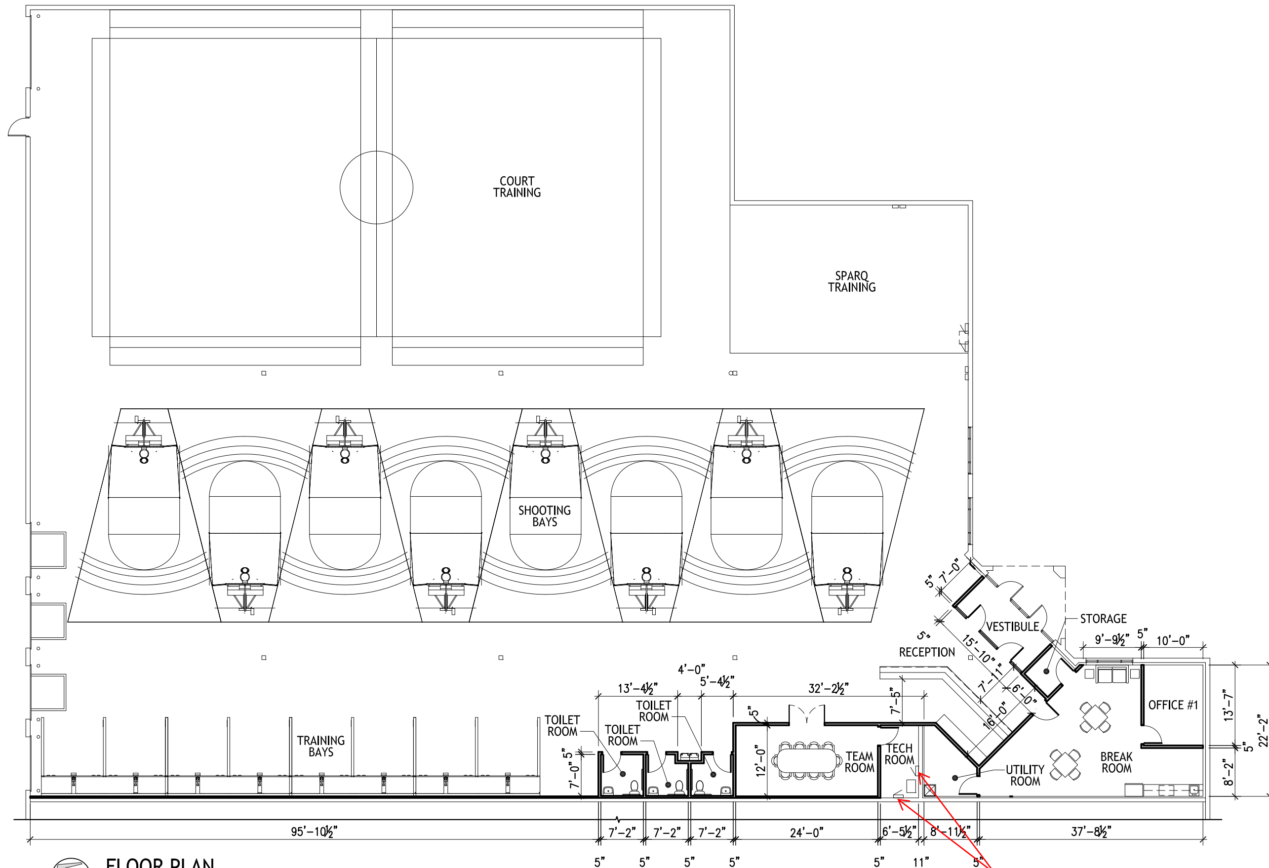
FLOOR PLAN 1/16" = 1'-0"
