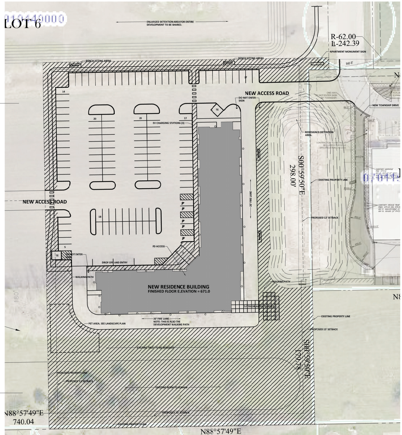
1 SITE PLAN 1" = 20'-0"
