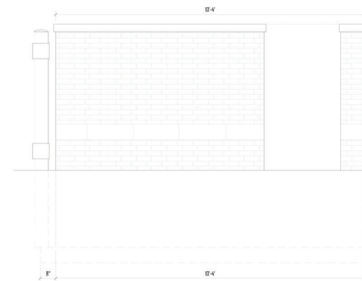
7 T.E. SIDE ELEVATION 3/8"=1'-0"
