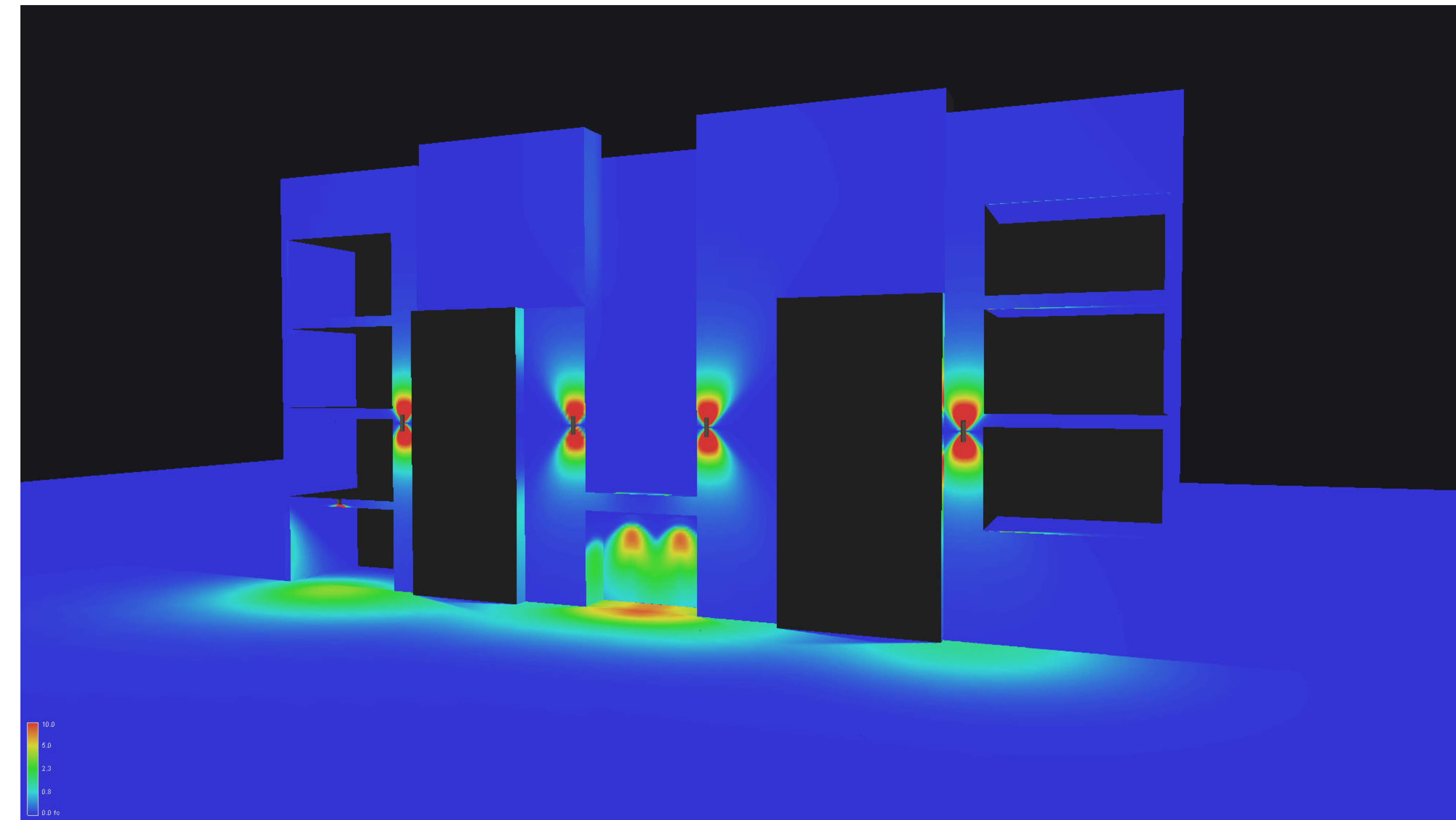
ILLUMINANCE (fc)
