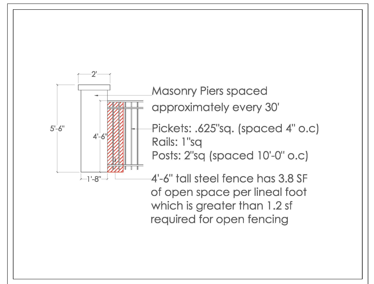
Fence Detail - Not to Scale
