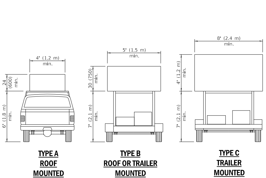
ARROW BOARDS
