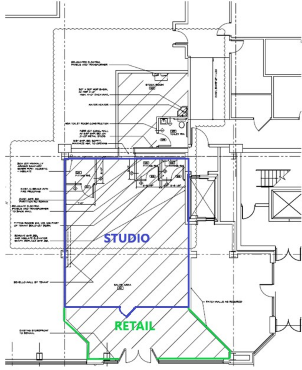
DEMOLITION / FLOOR PLAN SCALE: 1/4" = 1'-0"
