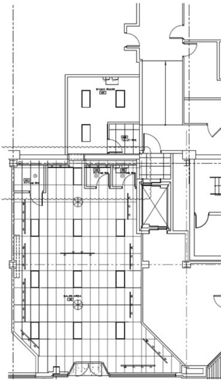
REFLECTED CEILING PLAN SCALE: 1/4" = 1'-0"
