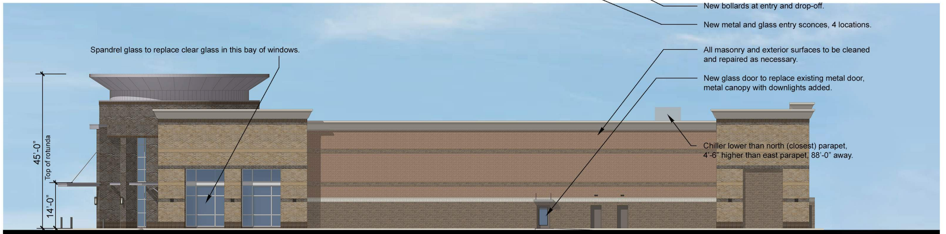
East Elevation
