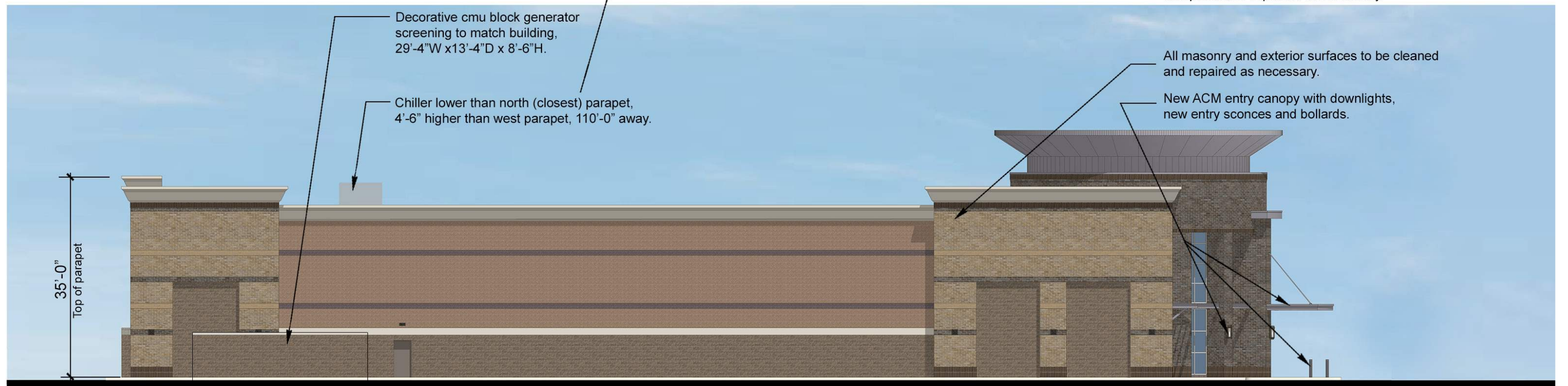
West Elevation
