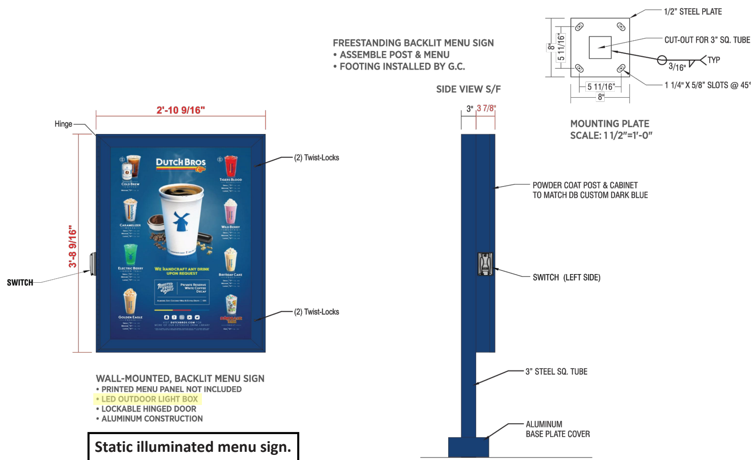
4 MENU BOARD - SINGLE, BY OTHERS - REFERENCE ONLY NOT TO SCALE
