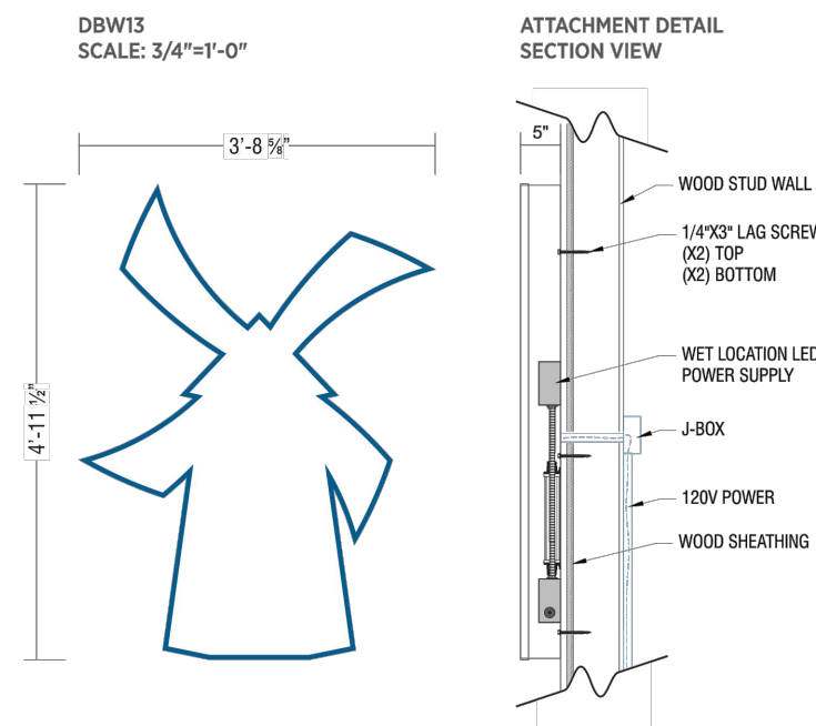
2 BUILDING SIGN, WINDMILL, BY OTHERS - REFERENCE ONLY NOT TO SCALE
