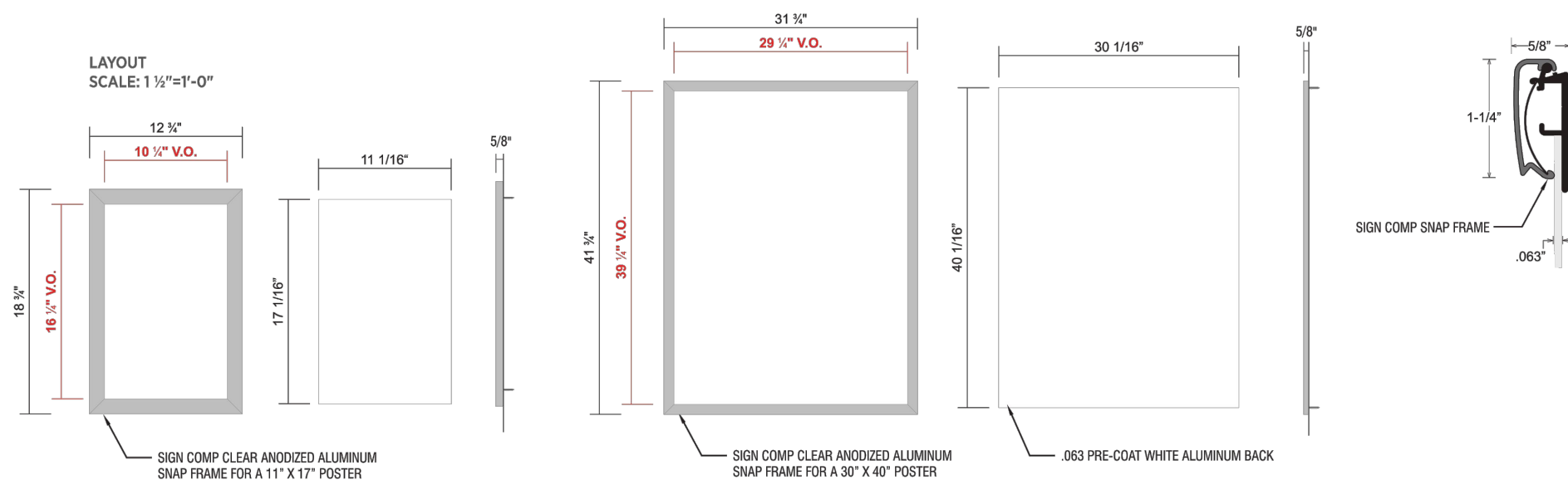
5 BUILDING SIGN, SNAP FRAMES, BY OTHERS - REFERENCE ONLY NOT TO SCALE
