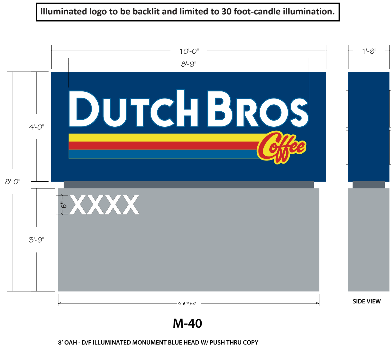
2 MONUMENT SIGN BY OTHERS - REFERENCE ONLY NOT TO SCALE
