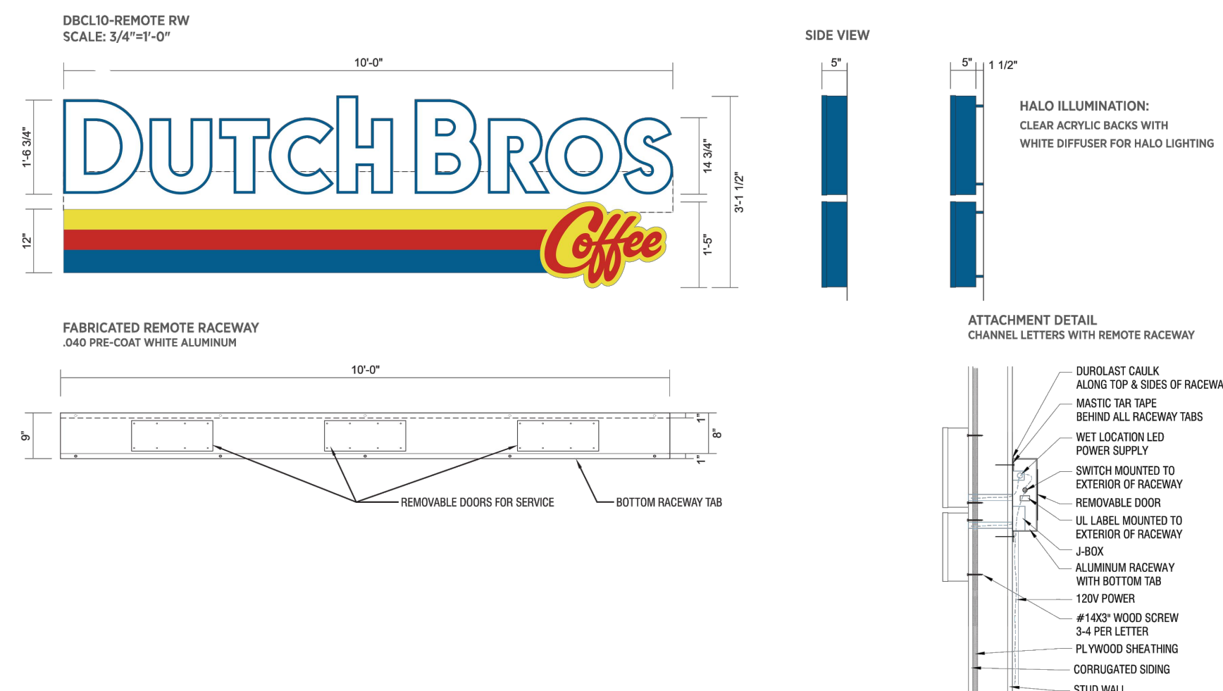
1 BUILDING SIGN, CHANNEL LETTERS, BY OTHERS - REFERENCE ONLY NOT TO SCALE
