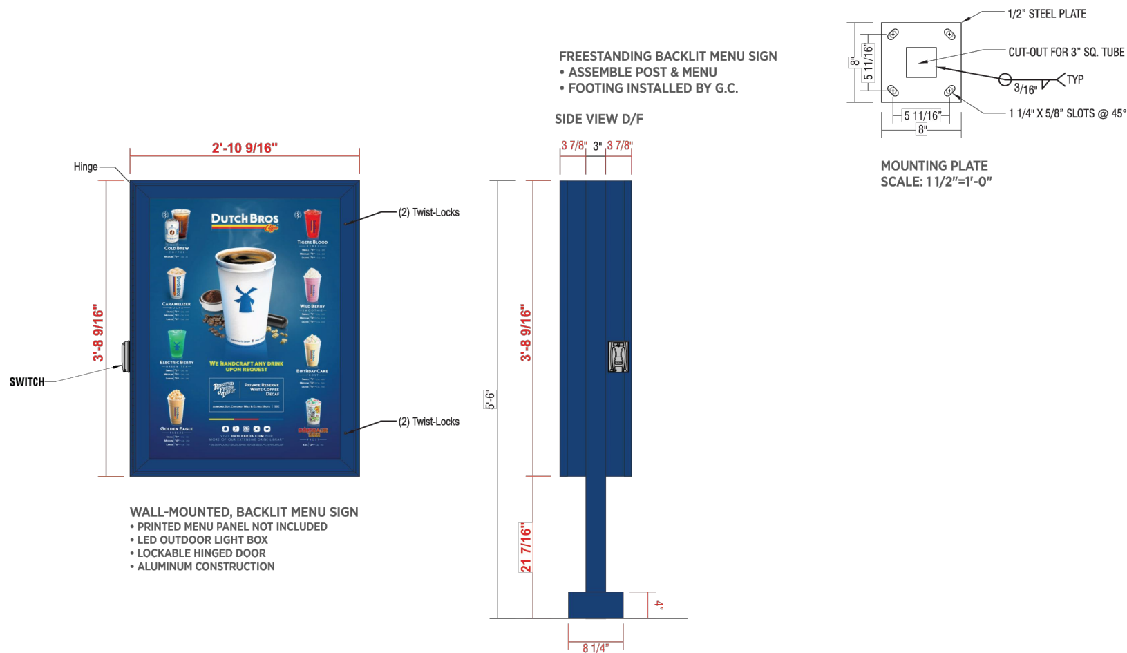
5 MENU BOARD - DOUBLE, BY OTHERS - REFERENCE ONLY NOT TO SCALE
