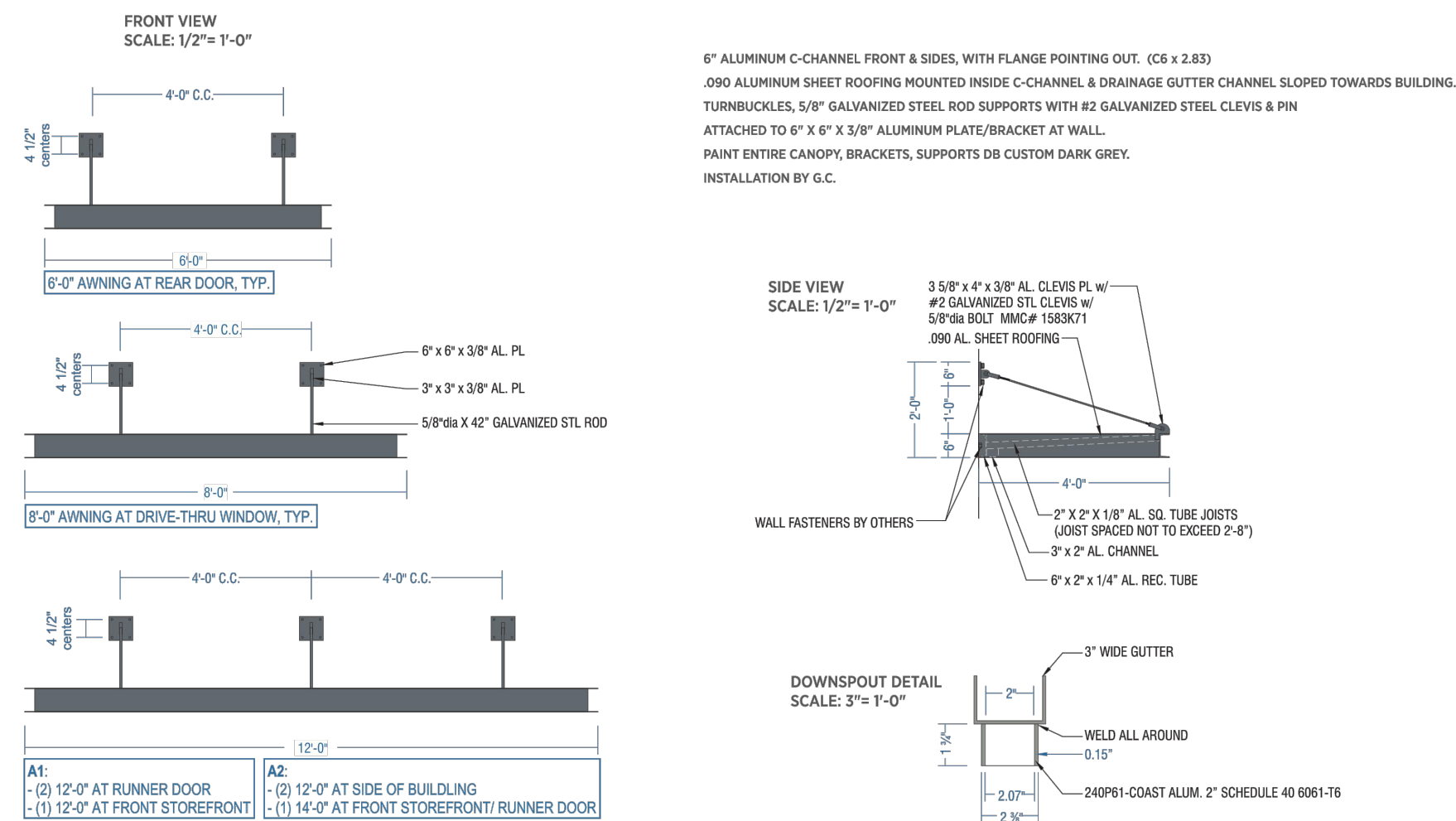
7 PRE-FAB. METAL AWNINGS BY OTHERS, - REFERENCE ONLY NOT TO SCALE
