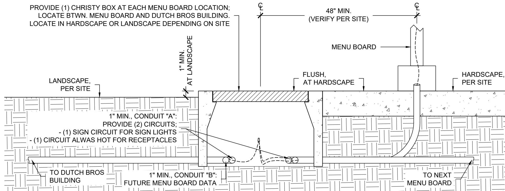
3 MENU BOARD & CHRISTY BOX DETAIL - REFERENCE ONLY NOT TO SCALE
