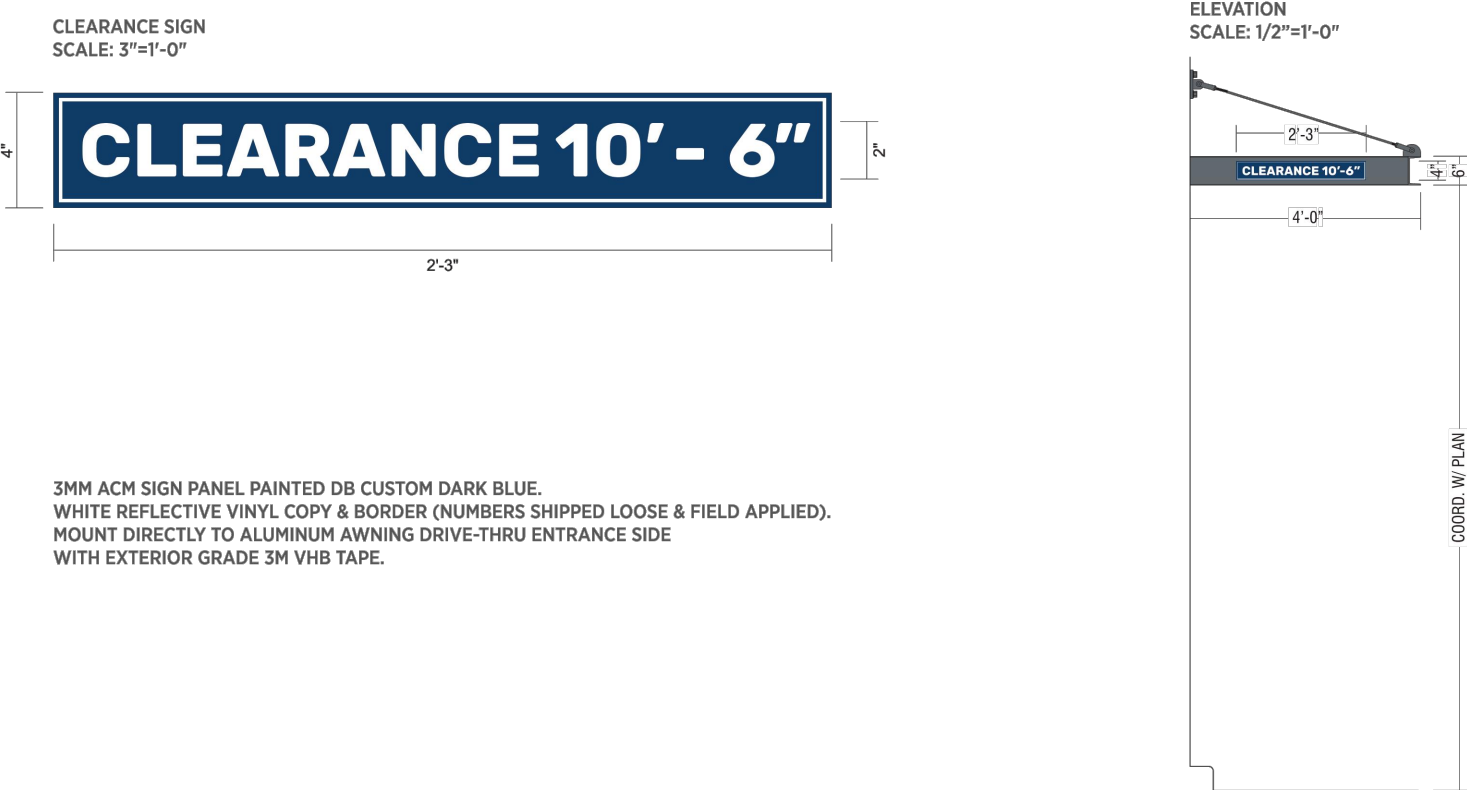
AWNING CLEARANCE SIGN, BY OTHERS AT DRIVE-THRU WINDOW - REFERENCE ONLY NOT TO SCALE
