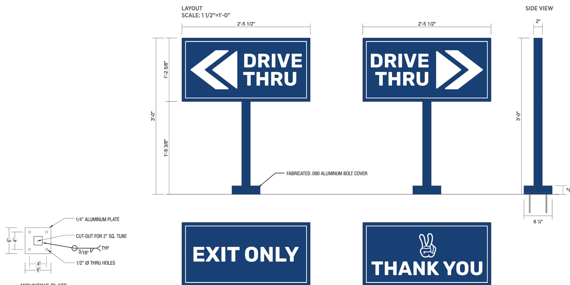
6 DIRECTIONAL SIGNS BY OTHERS - REFERENCE ONLY NOT TO SCALE
