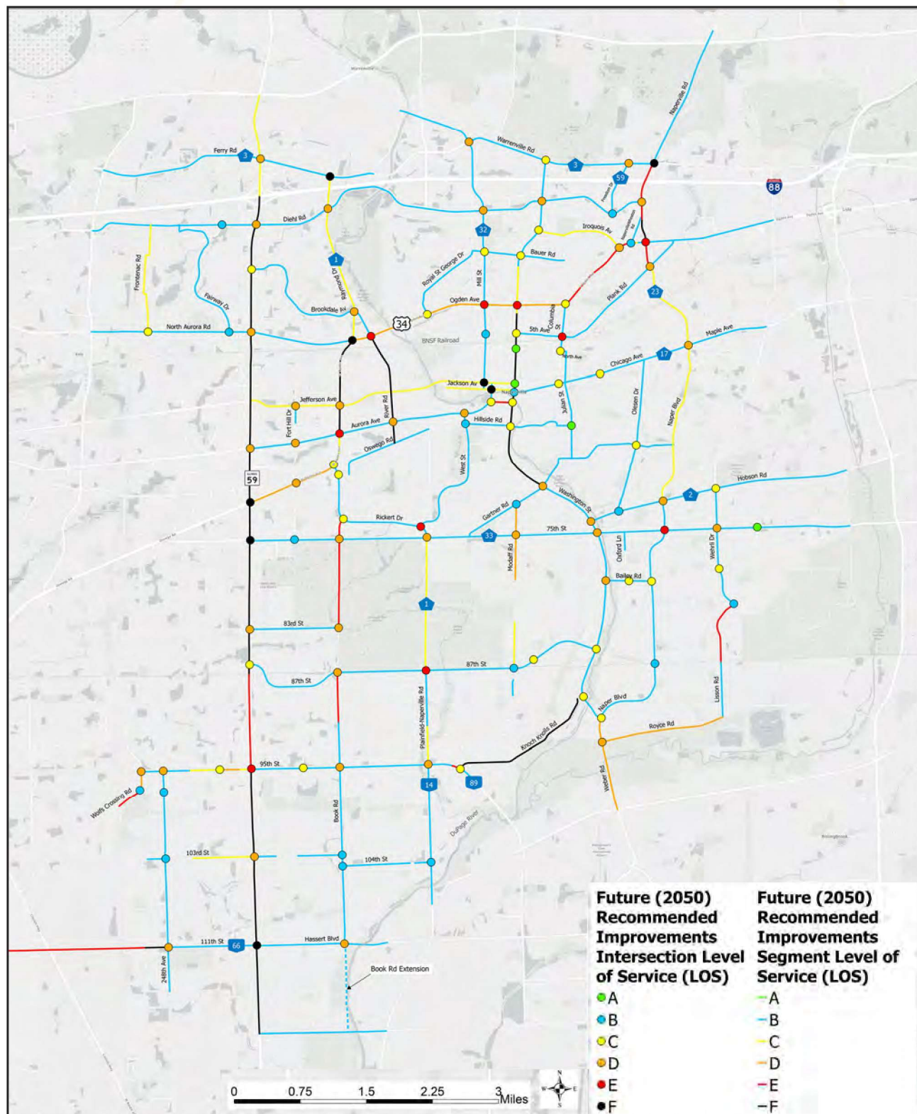
Summary of Future Year 2050 Level of Service with Capacity Improvements
