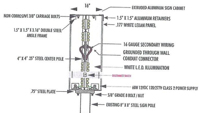
TYPICAL UL LISTED LED ILLUMINATED DOUBLE SIDED SIGN CABINET LED ILLUMINATION
