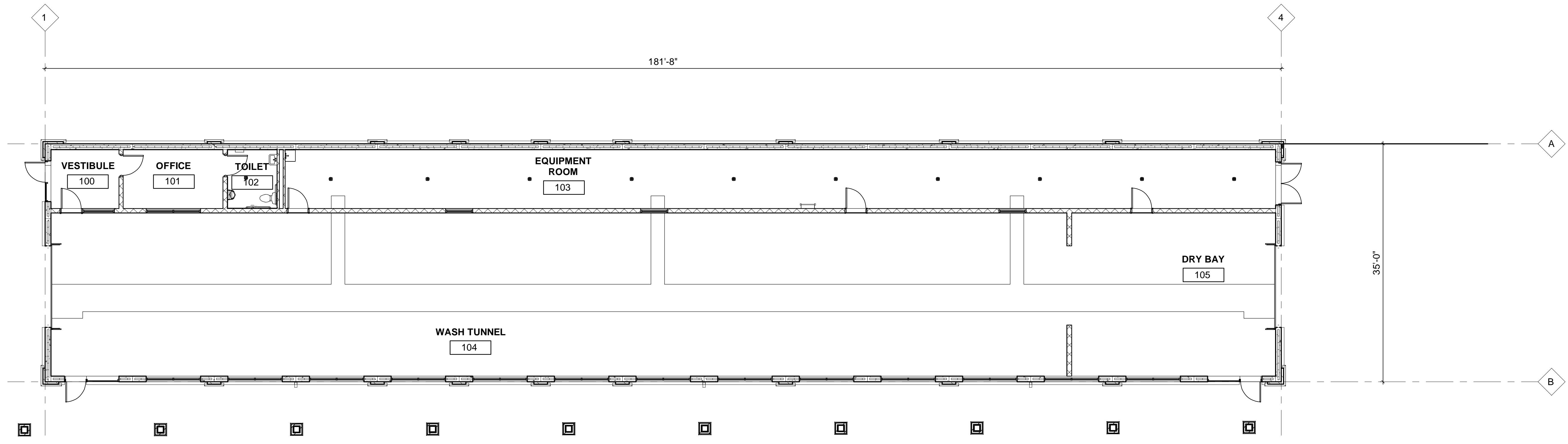
1 FLOOR PLAN 1/8" = 1'-0" 0 8 16 NORTH
