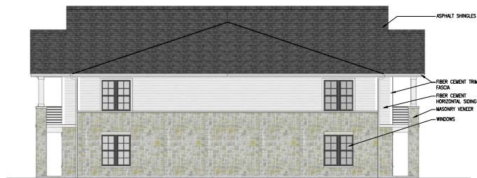
18 UNIT BUILDING - TYPE 'C' RIGHT ELEVATION 1/8" = 1'-0"
