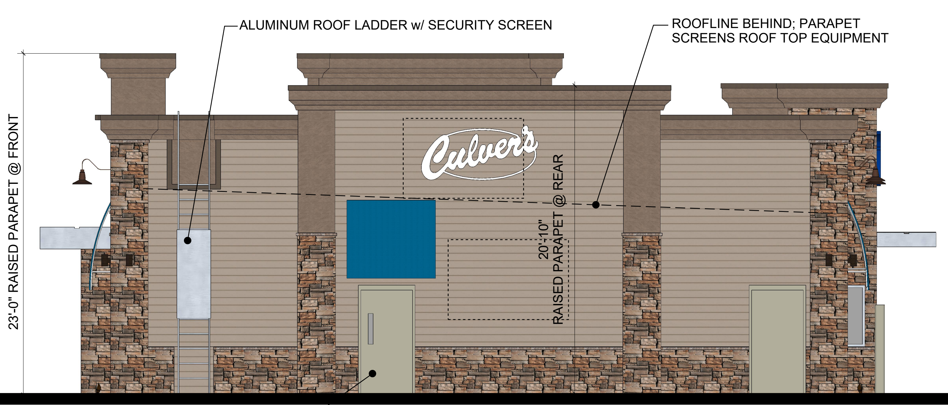
REAR ELEVATION
