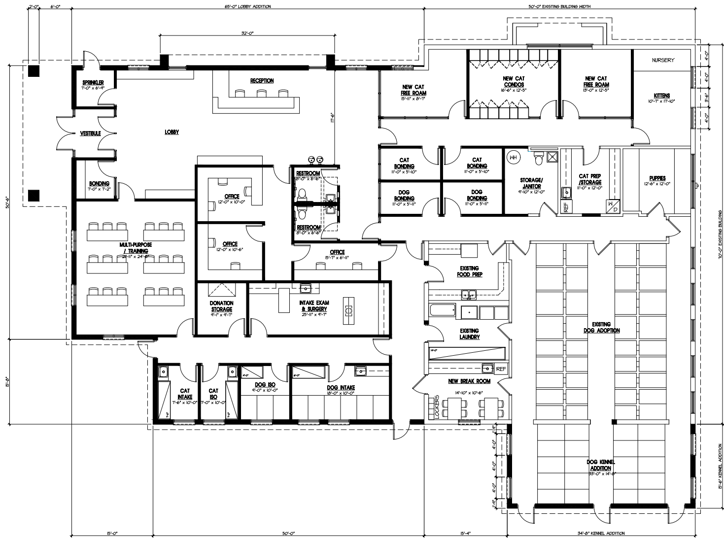
FLOOR PLAN 0 5 10 SCALE 3/8"=1'-0"
