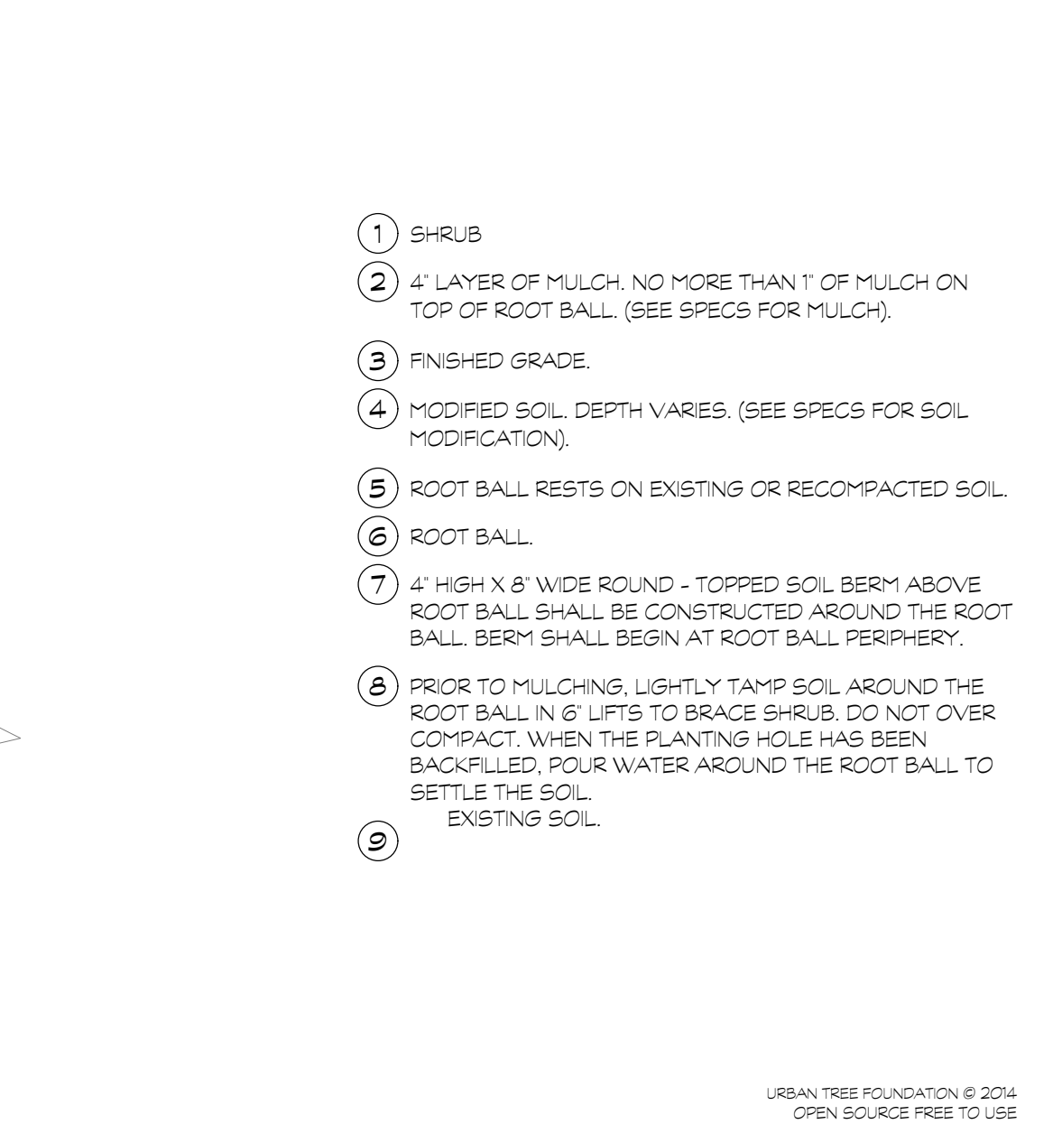
3 TREE W/ BERM (EXISTING SOIL MODIFIED) 1/2" ± 1'-0"
