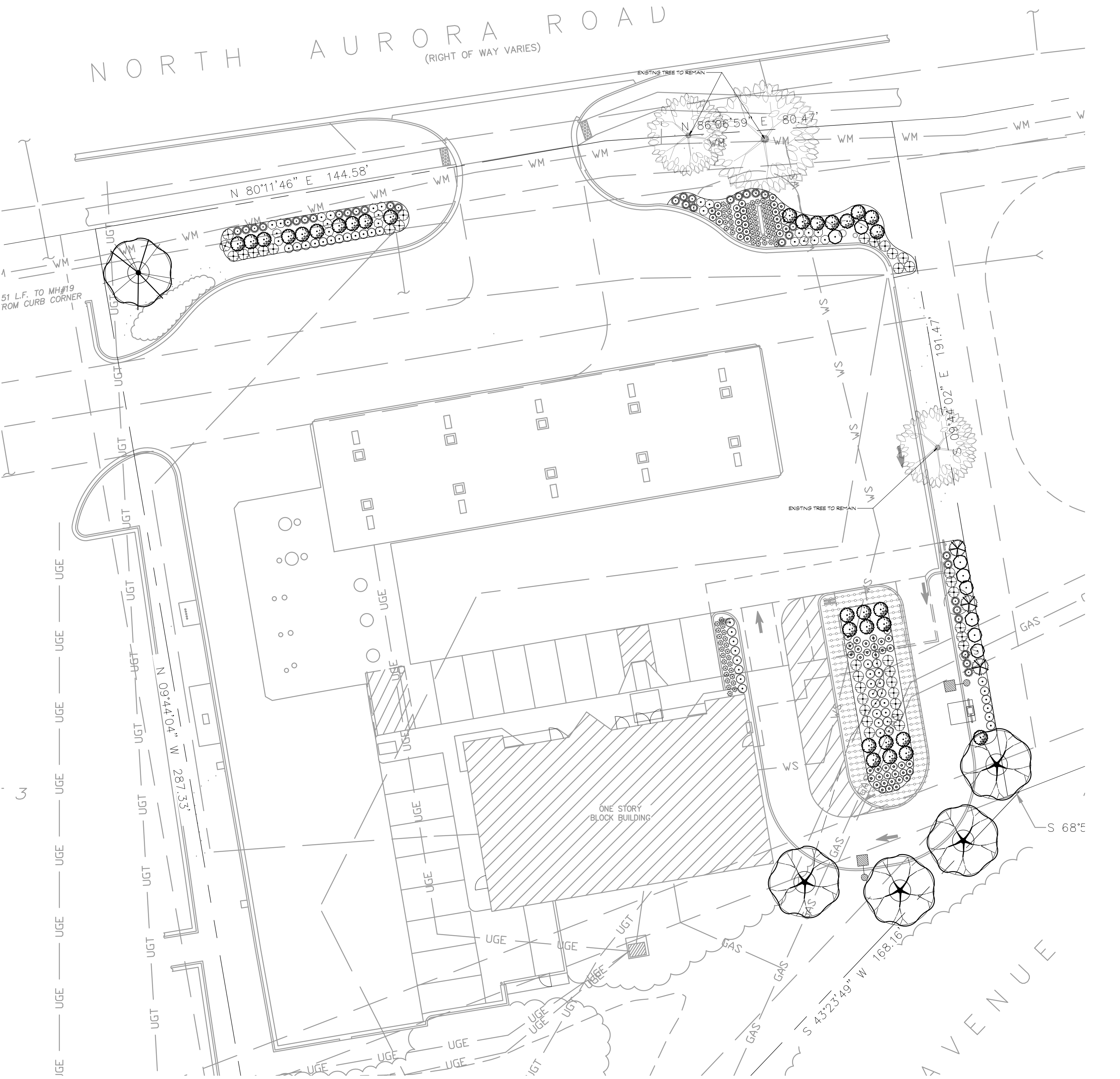
1 PROPOSED LANDSCAPE PLAN SCALE: 1" = 20'-0"
