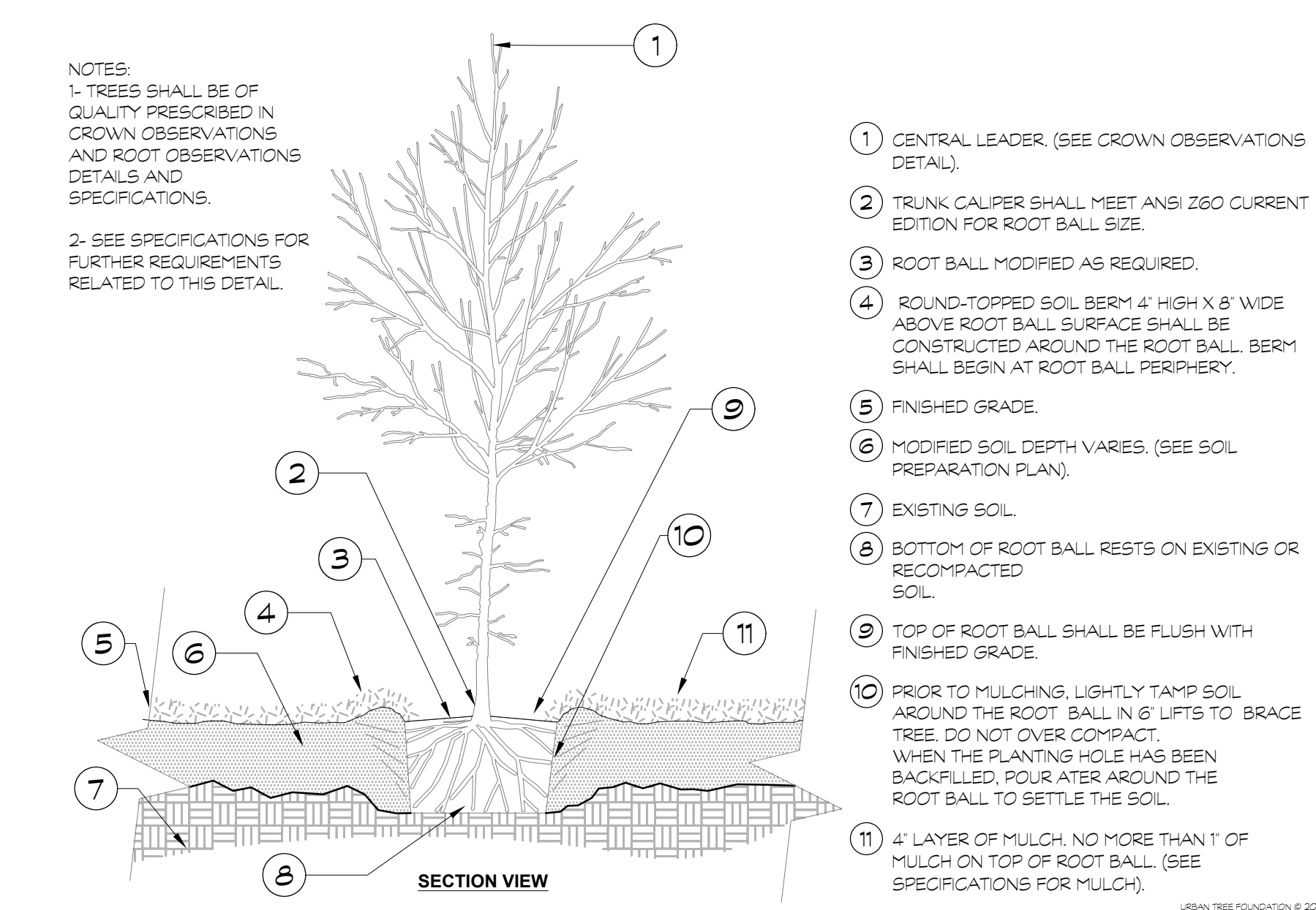
3 TREE W/ BERM (EXISTING SOIL MODIFIED) 1/2" ± 1'-0"
