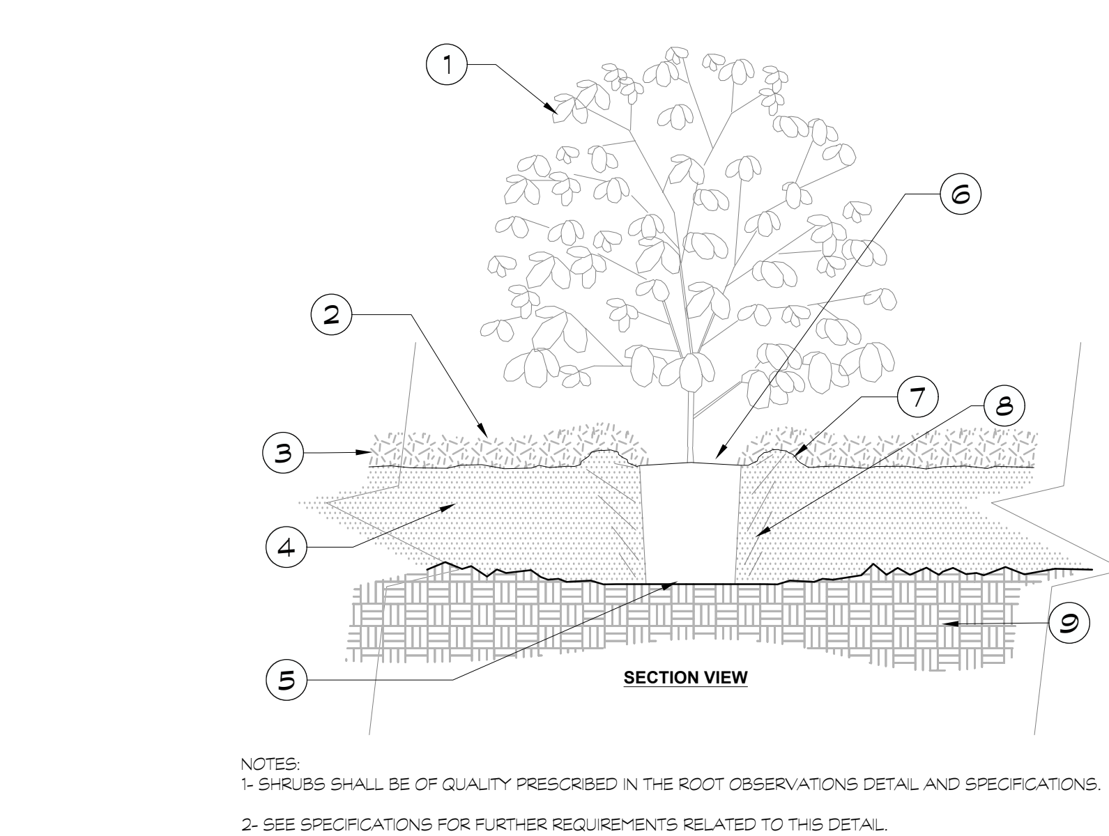
2 SHRUB - MODIFIED SOIL 3/4" ± 1'-0"
