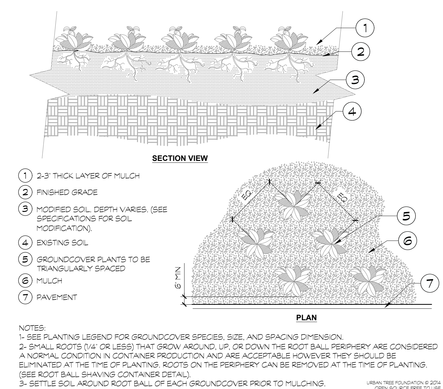
1 GROUND COVER 3/4" ± 1'-0"
