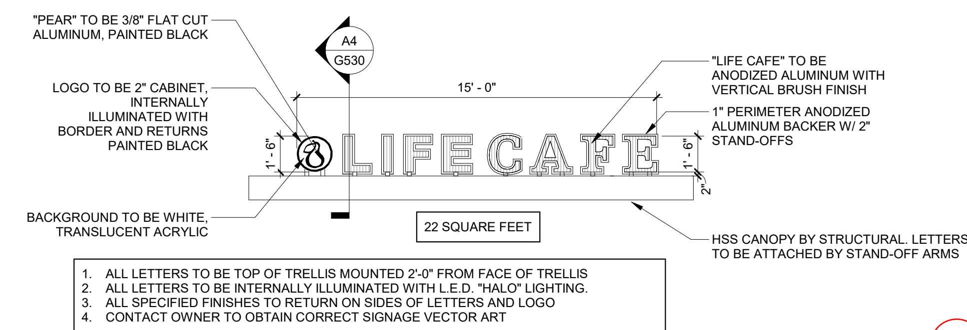
B1 SIGN "C" - LIFE CAFE SIGNAGE 1/4" = 1'-0"
