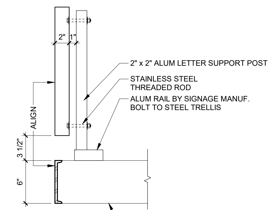
A5 CANOPY SIGN ATTACHMENT - TRELLIS 1 1/2" = 1'-0"
