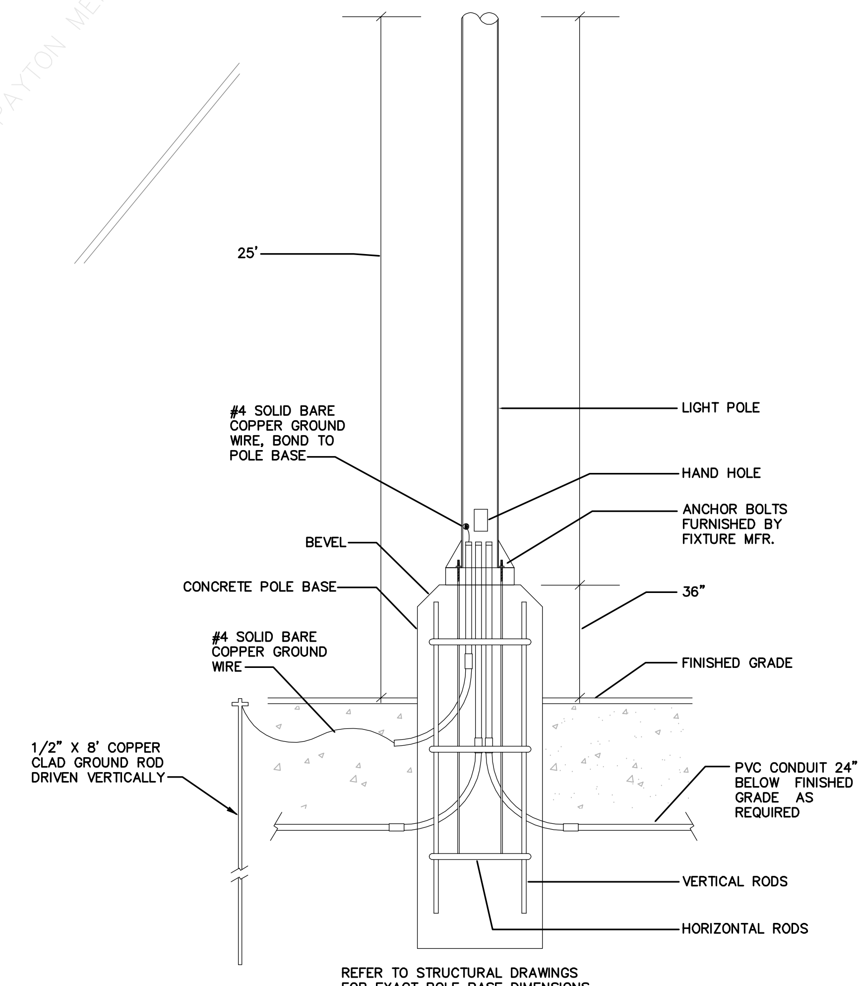
2 TYPICAL POLE BASE DETAIL NOT TO SCALE
