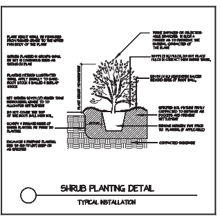
DECIDUOUS TREE PLANTING DETAIL TYPICAL INSTALLATION - 3" (75MM) CALIPER OR LESS
