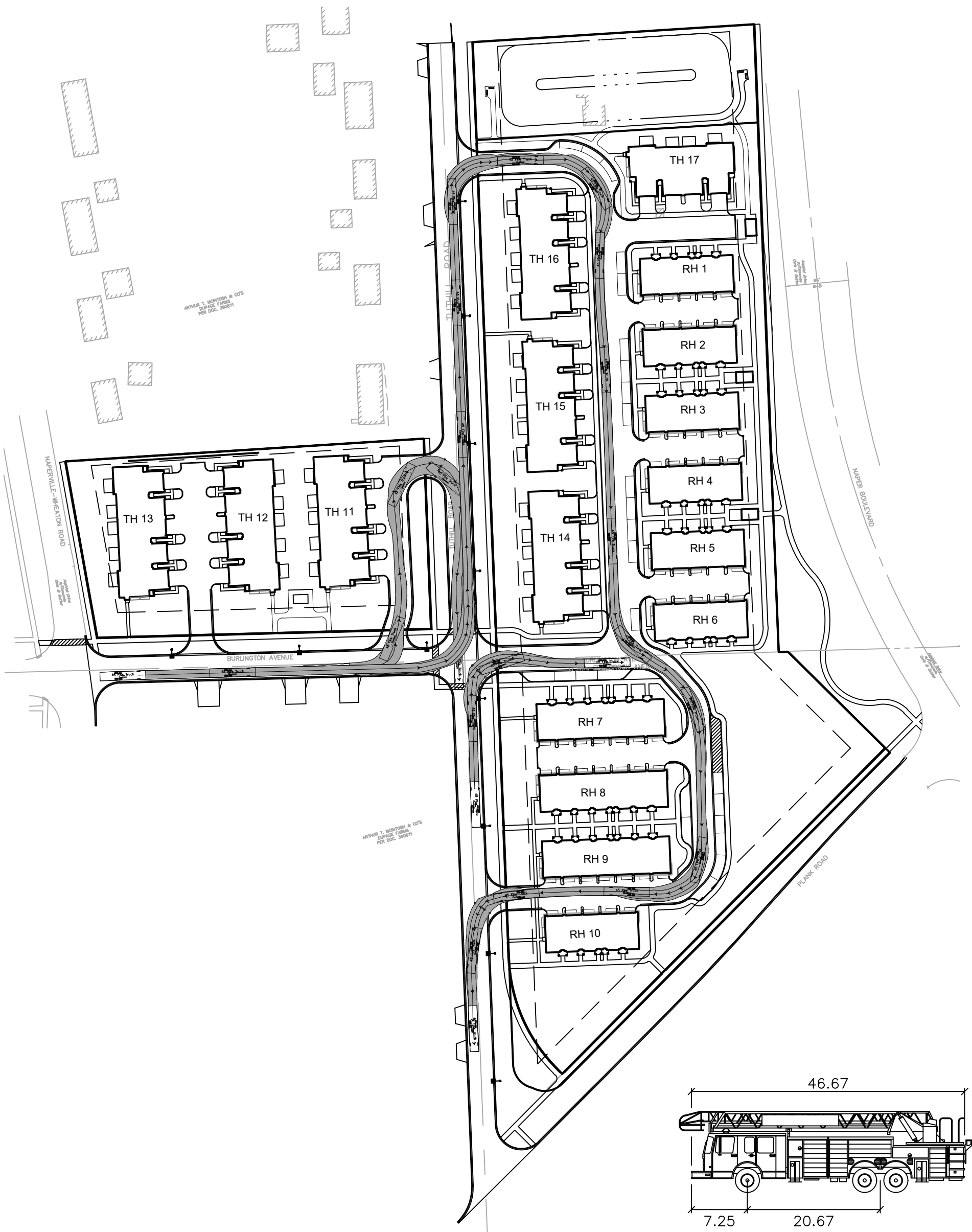
45 FIRE TRUCK
