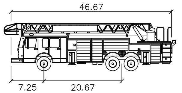
45 FIRE TRUCK
