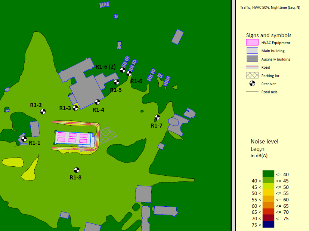
Figure 4: Nighttime Leq of HVAC and Traffic Model
