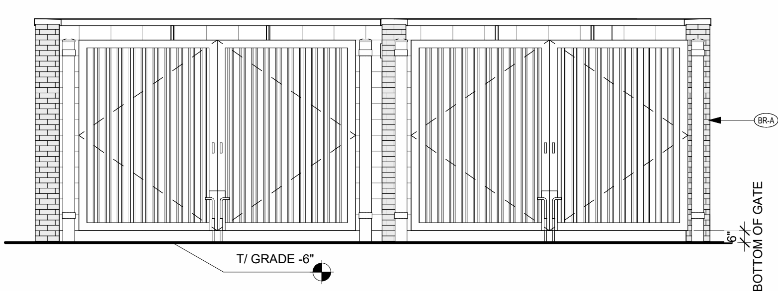
1 REFUSE ENCLOSURE WEST ELEVATION N.T.S.
