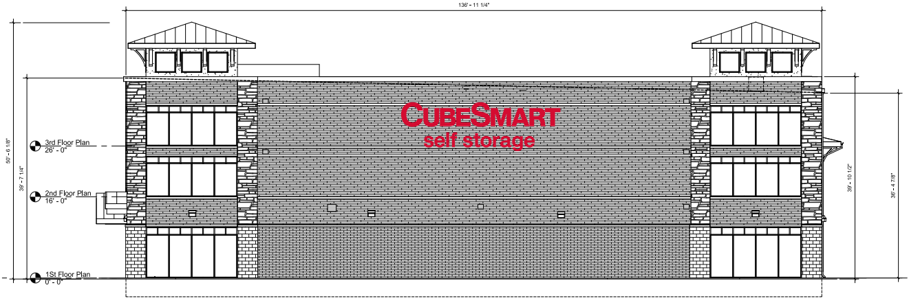
West Elevation 1/8" = 1'-0"
