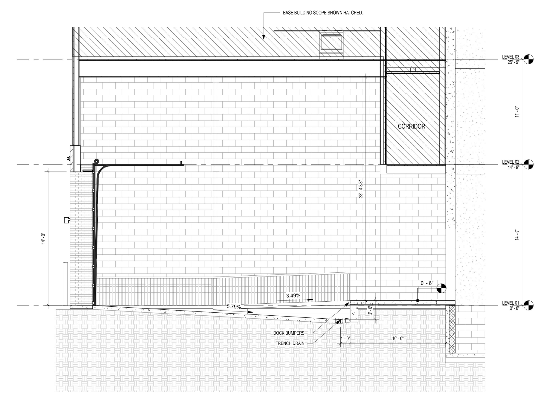
2 EVENT SPACE DOCK SECTION
