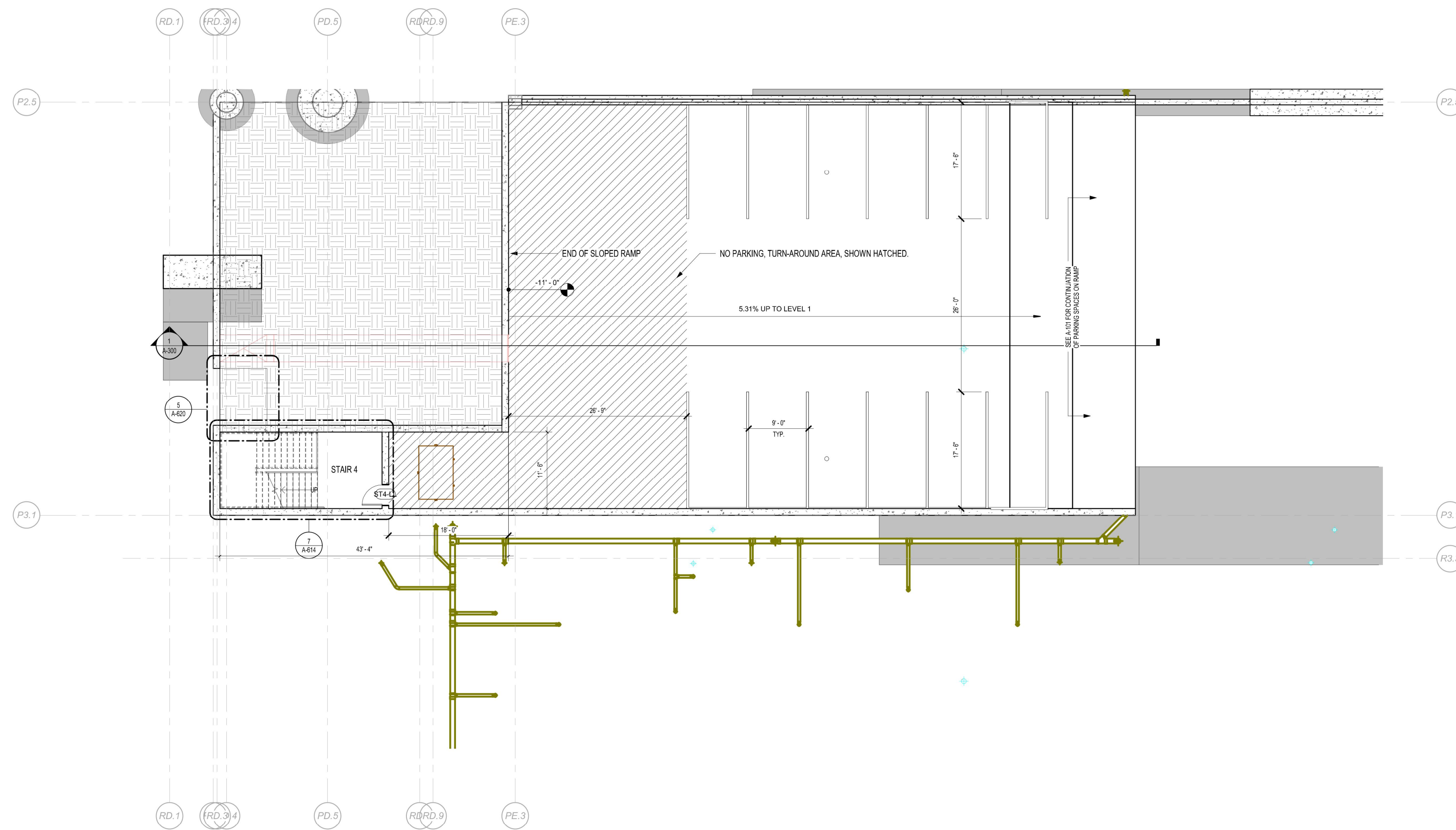
① LOWER LEVEL FLOOR PLAN
