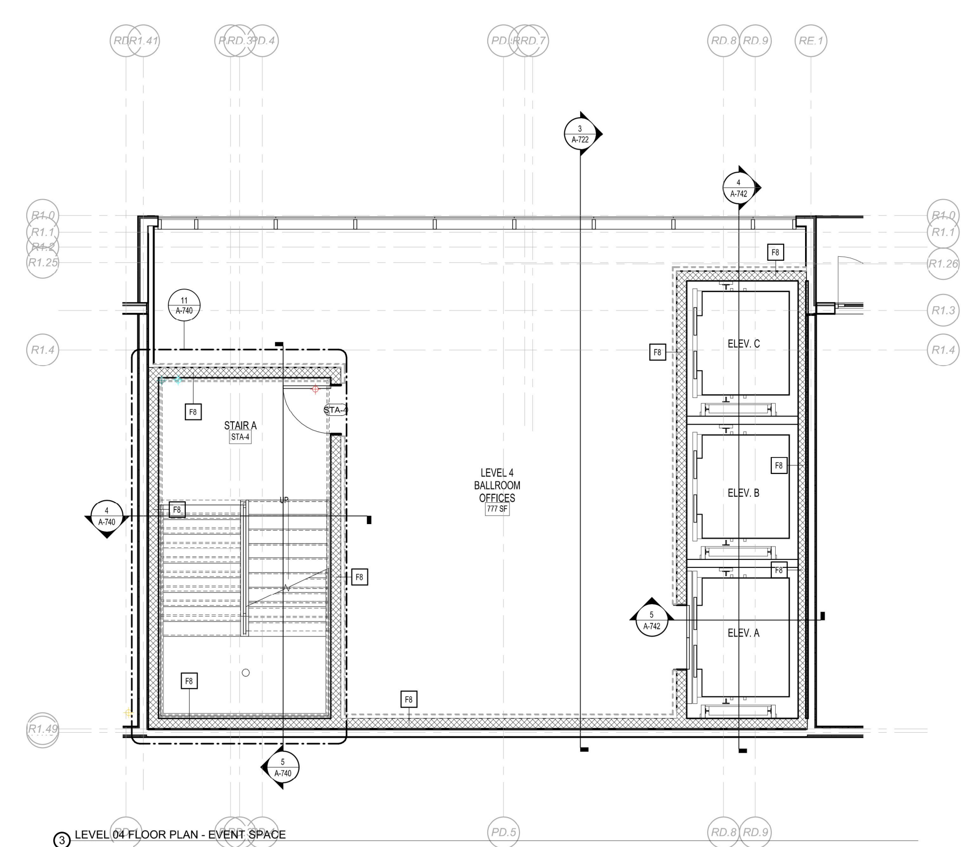
3 LEVEL 04 FLOOR PLAN - EVENT SPACE
