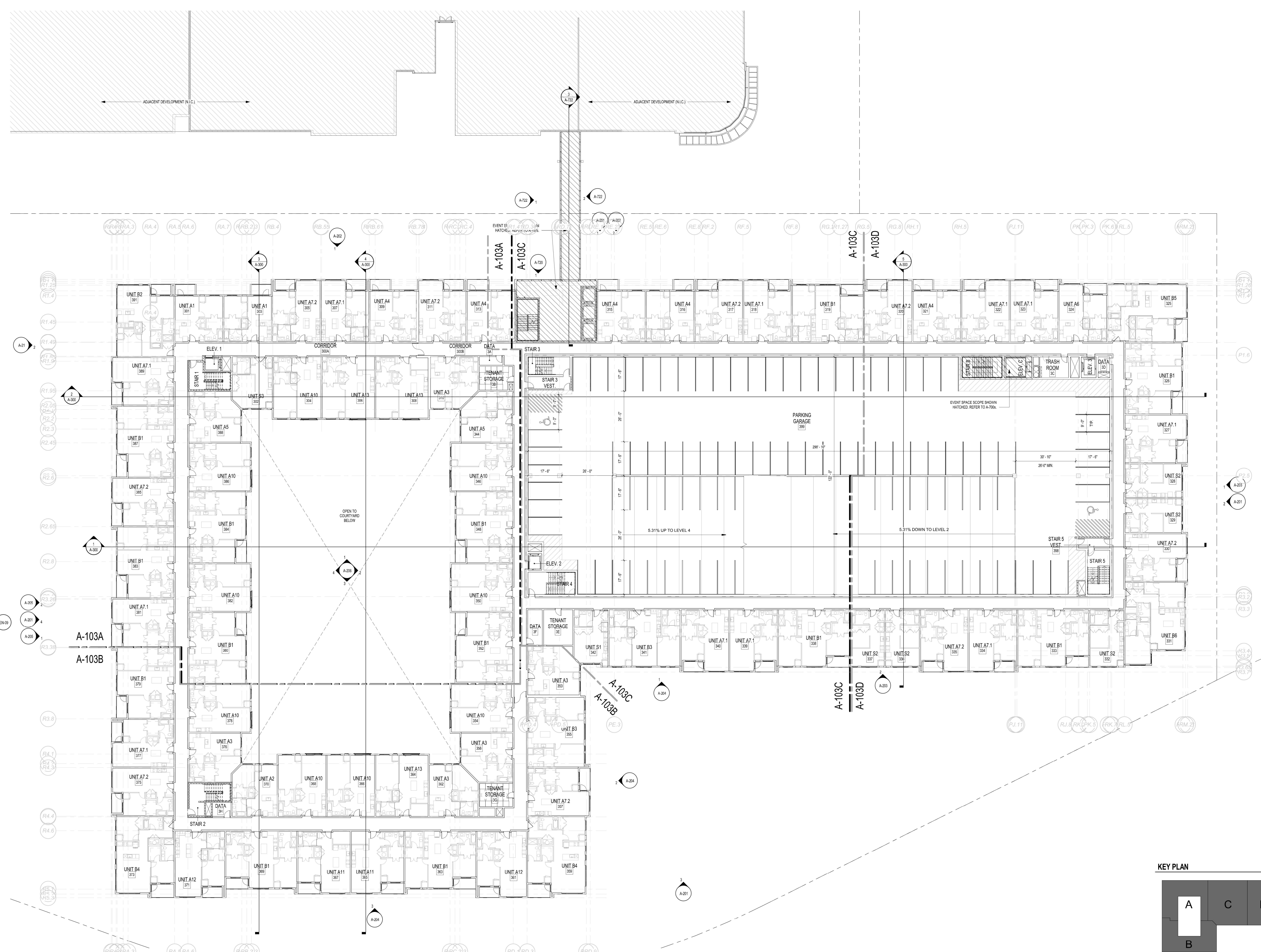
LEVEL 03 FLOOR PLAN - OVERALL
