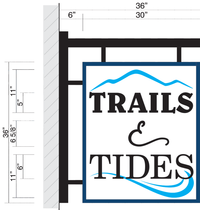
NON-ILLUMINATED D.F. CUSTOM BLADE SIGN DISPLAY SCALE: 1 1/2" = 1'-0" SIGN #2 QTY. 1 2" DEEP WHITE FORMED PANEL W/ 1" DEEP POLYCARBONATE LETTERS PAINTED BLACK. BACKGROUND GRAPHICS TO BE LIGHT AND DARK BLUE VINYL GRAPHICS APPLIED TO D.F. PANEL.
