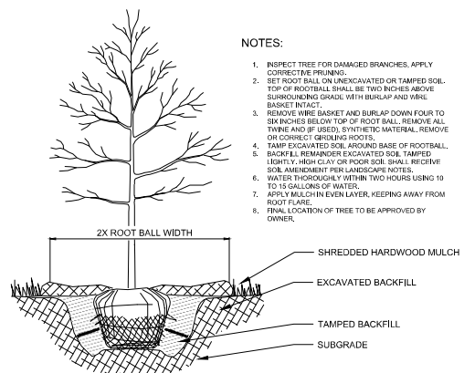
1 TREE PLANTING NTS
