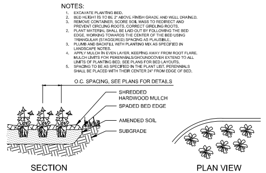
3 PERENNIAL PLANTING NTS
