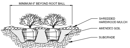
2 SHRUB PLANTING NTS
