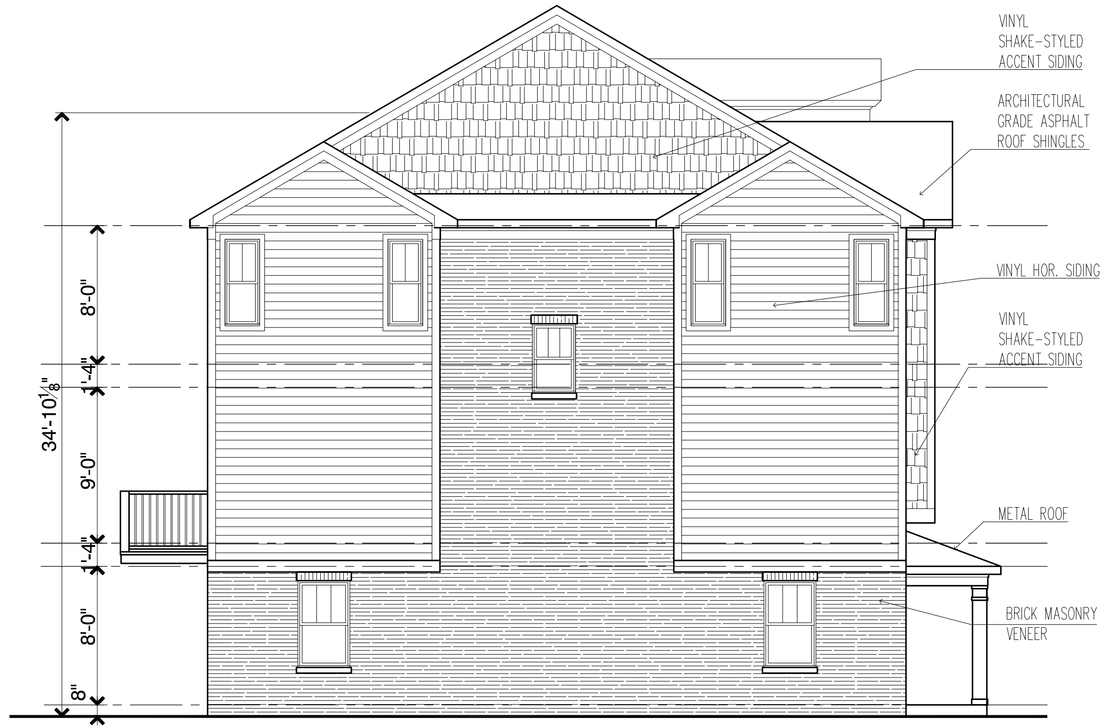
PLANK ROAD LEFT ELEVATION
