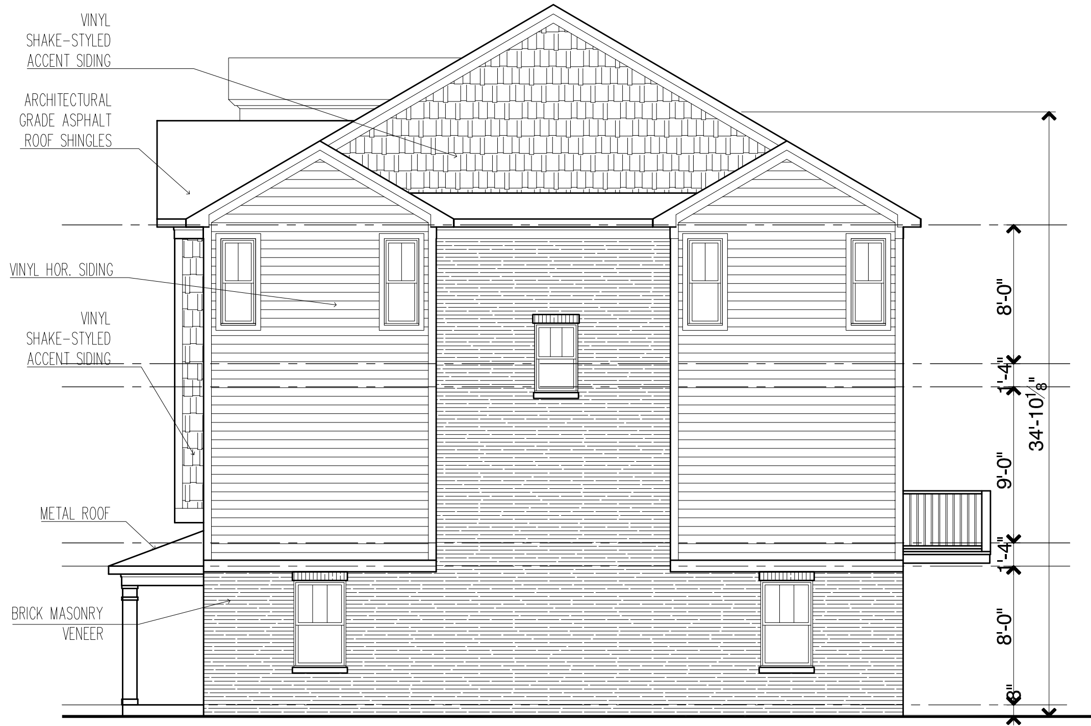
PLANK ROAD RIGHT ELEVATION
