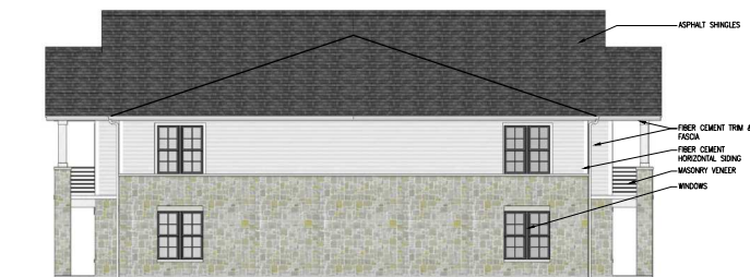
22 UNIT BUILDING - TYPE 'A' LEFT ELEVATION 1/8" = 1'-0"
