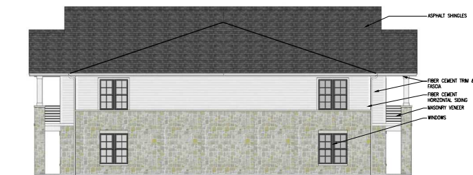
22 UNIT BUILDING - TYPE 'B' LEFT ELEVATION 1/8" = 1'-0"
