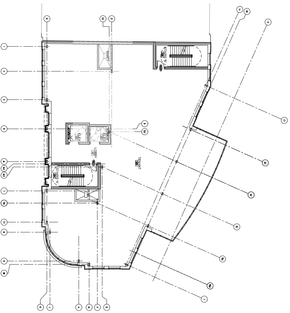
SECOND FLOOR PLAN SCALE: 1/8" = 1'-0" 6/5/20 GF
