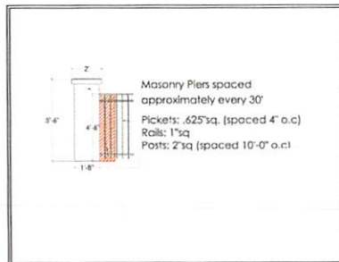
Fence Detail - Not to Scale
