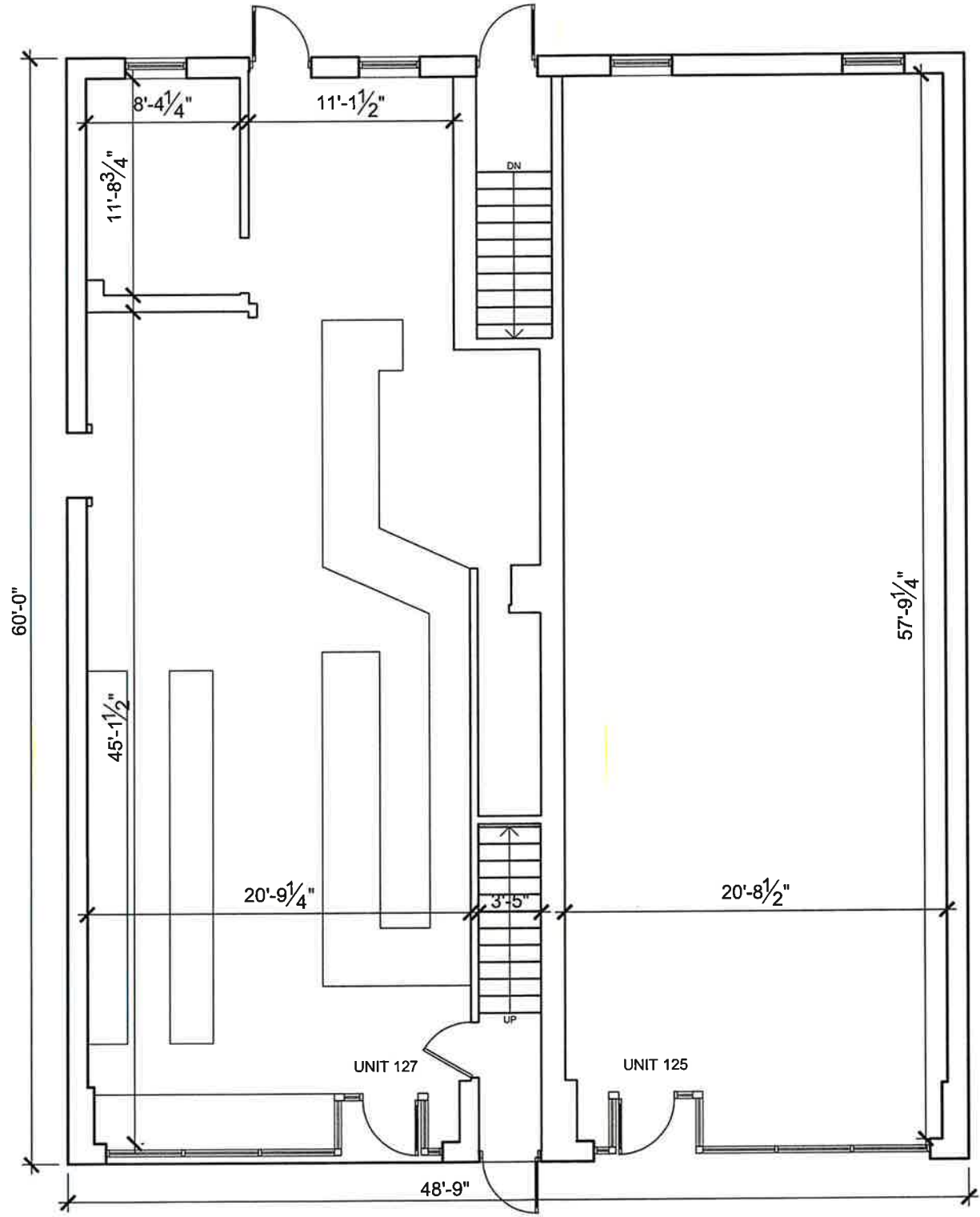
N 1 FIRST FLOOR PLAN 1/8" = 1'-0"
