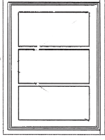
As Viewed From The Exterior FS 36 3/4" X 24 11/16" RO 37 3/4" X 25 3/16"
