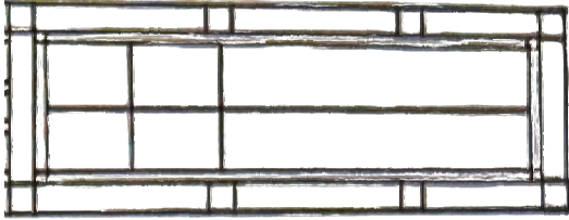
As Viewed From The Exterior FS 29 3/8" X 57 5/16" RO 30 3/8" X 57 13/16"
