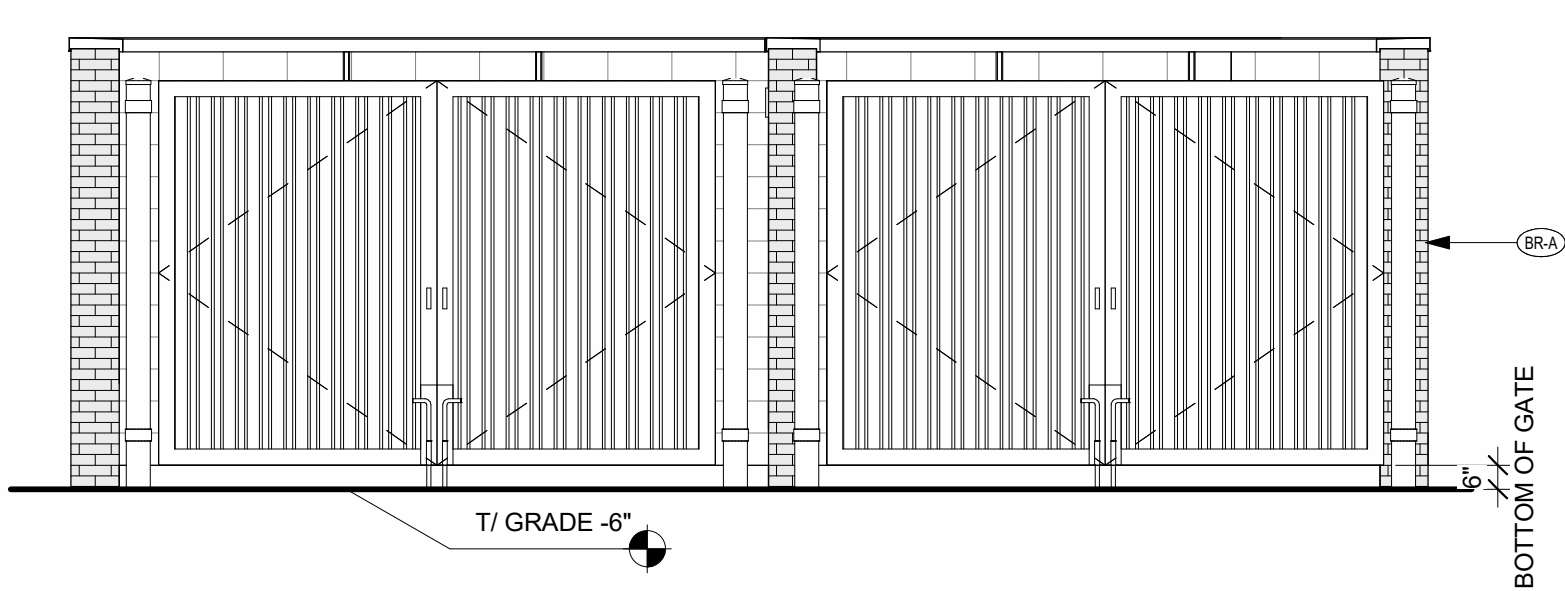
1 REFUSE ENCLOSURE WEST ELEVATION N.T.S.
