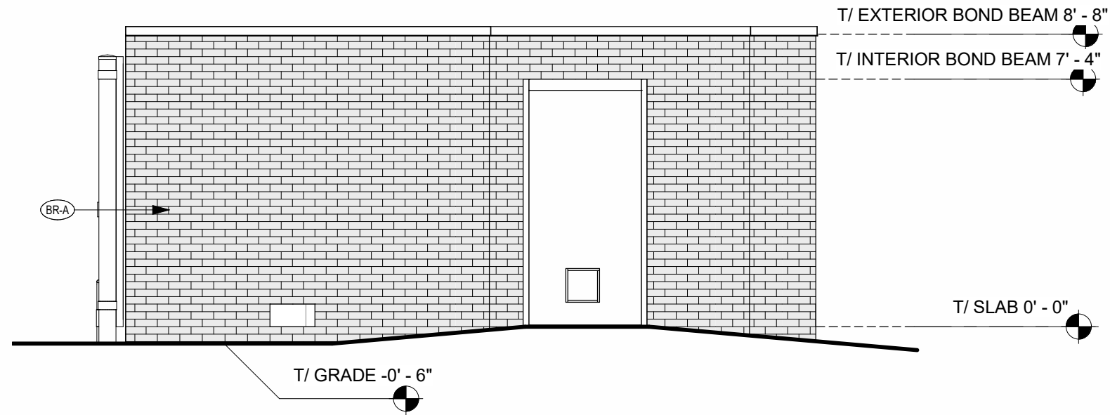
2 REFUSE ENCLOSURE SOUTH ELEVATION N.T.S.
